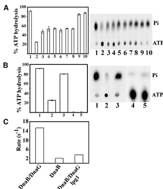
Figure 3. Thin-Layer Chromatography-Based ATPase Assays
